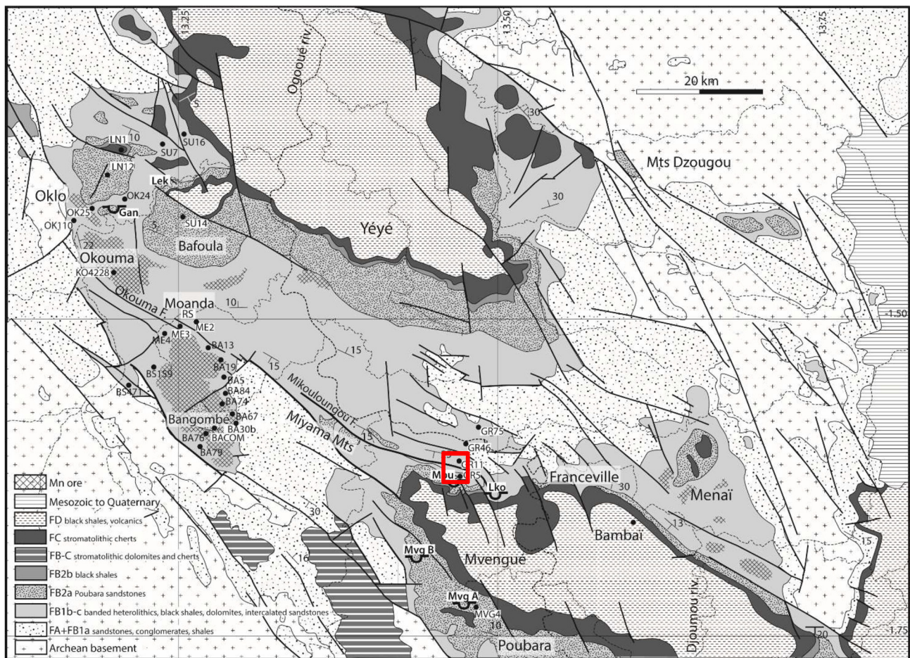
Fig. 1. Geological map of the Franceville Basin. The studied outcrops are located in the Moulende quarry (red square). Structural framework and unit contours modified from Weber (1968) and Gauthier-Lafaye (1986).
