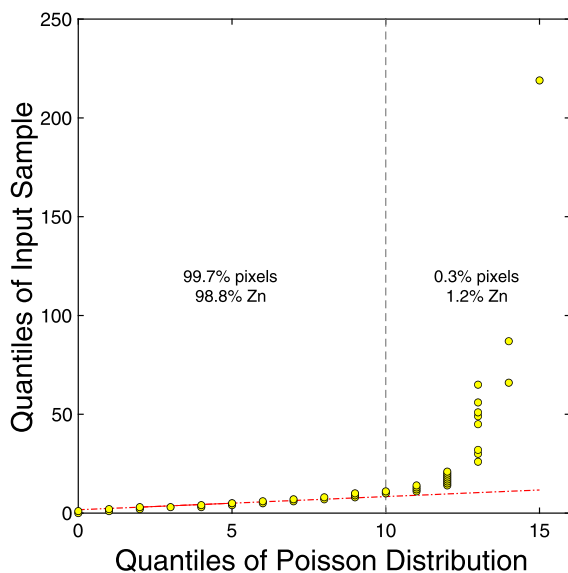
Fig. 8. Quantile-quantile plot comparing, as an example, the observed frequency of the Zn intensity (counts per 10 ms per pixel) measured in the fillings by SR-XRF (shown in Fig. S4) with the frequencies expected from a Poisson (random) distribution. The 1:1 straight-line (in stippled red) shows the perfect correspondence for low-counts pixels, which are the overwhelming majority. The array deviates from linearity at \sim 10 cps. Only 0.3% of the pixels are outliers ( >10 cp 10 ms) with respect to a Poisson distribution and they account for 1.2% of the total Zn concentration of the measured region. The bulk of the Zn inventory, and in particular Zn excesses, therefore should be associated with the carbon-rich background matrix and not with disseminated sulfide crystals. Poisson distributions with similar (Zn outlier)/(total Zn) ratios were found for all the measured regions.
