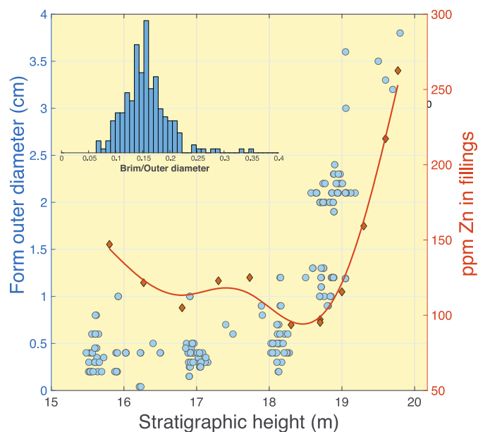
Fig. 5. Lenticular form diameters (in blue) and Zn contents of their fillings (in red) vs stratigraphic height. Jitter has been applied to the x-axis for better readability. The red curve is a fit of the filling data with a smoothing spline. The sharp increase of both parameters starting at 18.5 m indicates that a sudden increase in nutrient supply contributed to the ten-fold increase in organism size. Inset: Histogram of the brim/external diameter ratio, which shows that the geometric characteristics of the LF remain in constant proportion, a feature indicative of a biological origin.
