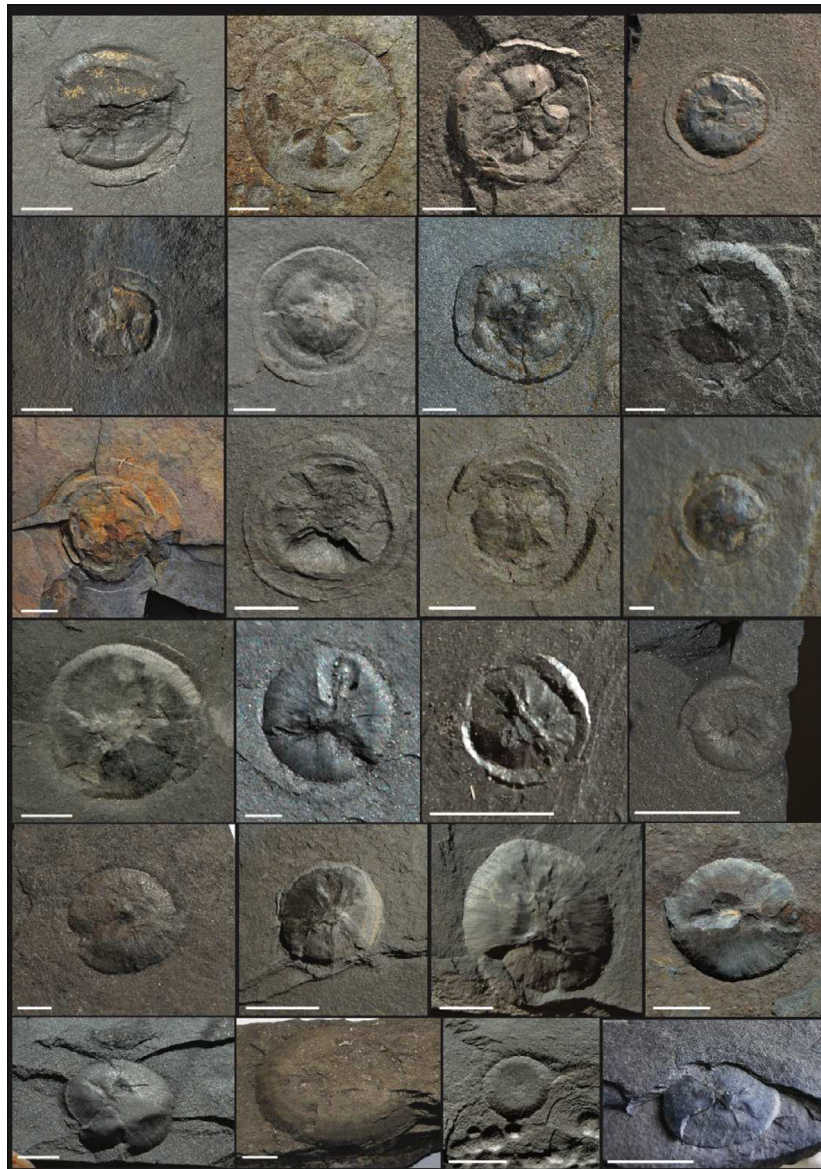
Fig. 3. Plate of 24 photographs of lenticular forms (LF) embedded in their black shale host rock (from subunit FB2b) arranged in a (row \times column) array. Scale bars represent 1 cm. The morphology is lenticular, occasionally segmented by radial structures (e.g., 1 \times 2 , 1 \times 3 , 3 \times 1 , 4 \times 1 ), and the outline is circular. A brim is present in some of the specimens (e.g., 1 \times 1 , 1 \times 2 , 1 \times 4 , 2 \times 2 , 3 \times 2 ). Other samples miss the brim (e.g., 5 \times 3 , 5 \times 4 , 6 \times 1 , 6 \times 3 ). This dichotomy may represent a contrast between the bottom and the top of the organism or be a preservation artefact. The dome part is filled with organic-rich clay.
