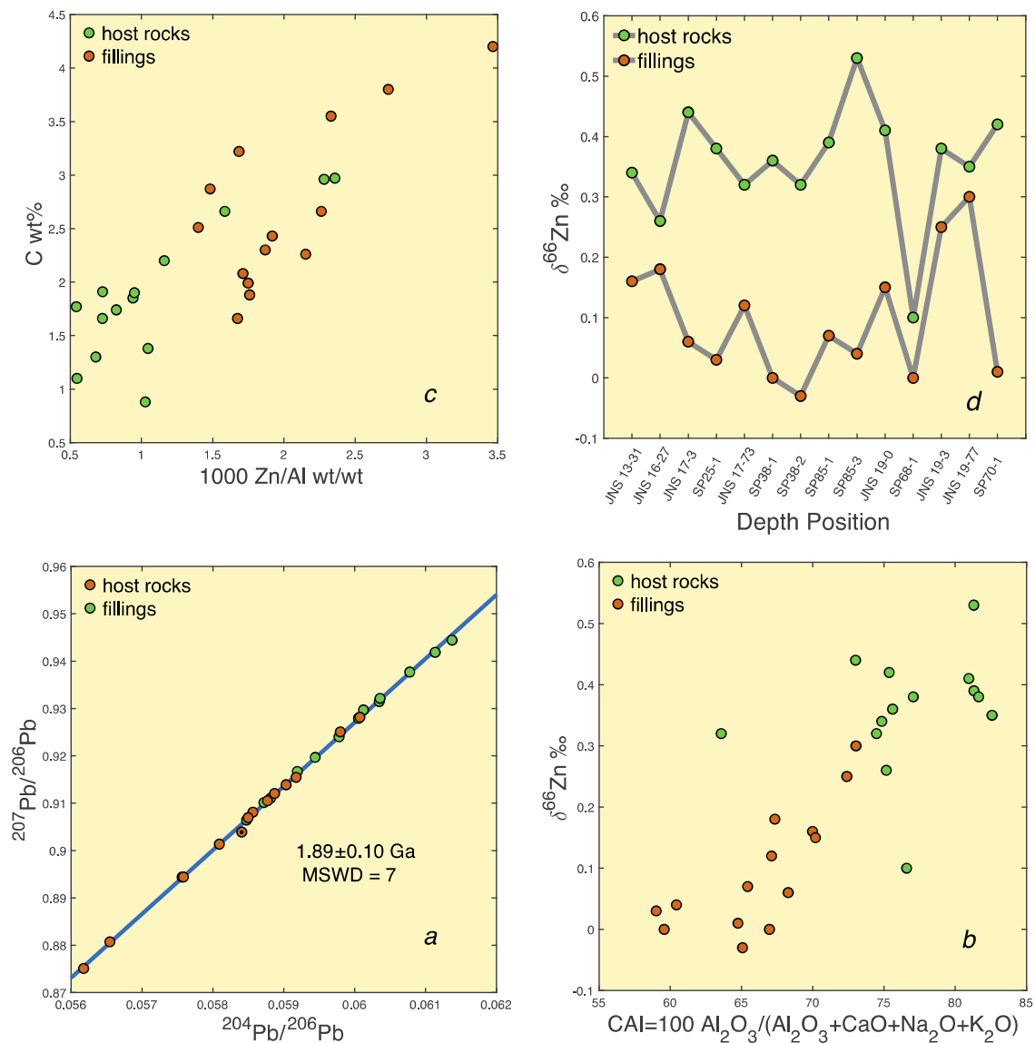
Fig. 7. Geochemistry of the host rock of the LF and their fillings. (a) The Pb-Pb linear array (inverse isochron) shows that if the U-Pb chronometer has been reset, it could only have been shortly after sedimentation. The sample with a bull's eye symbol has been left out of the calculations. The error bar includes correction for an MSWD value of 7 and is identical at the same confidence level to the errors calculated by Monte Carlo and bootstrapping. The age is indistinguishable from literature dates (Bonhomme et al., 1982; Bros et al., 1992). (b) Relationship between \delta^{66}\text{Zn} and the Chemical Index Alteration (CIA) (Nesbitt and Young, 1982). The host rock is dominated by residual material from thoroughly leached soils, whereas the LF fillings contain large fractions of fine-grained material (clays) eroded from the continental surface. (c) Correlation between the organic carbon contents of the host rock and the fillings and Zn/Al ratios. The main Zn carrier is clearly associated with the organic component. (d) Comparison between the \delta^{66}\text{Zn} values of the host rock and the corresponding LF fillings. The \delta^{66}\text{Zn} values of the host rock fall within the lithogenic range ( 0.28 \pm 0.13 ‰ (Moynier et al., 2017)), whereas the fillings are characterized by significantly lower \delta^{66}\text{Zn} indicative of organic carbon sediments (Little et al., 2016). Typical error bars are 0.05‰.
