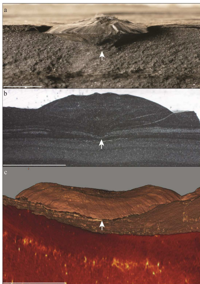
Fig. 4. (a) Biconvex LF specimen surrounded by its host rock. White arrows in all panels show the upper and lower apex, respectively. Scale bars in all panels are 1 cm. (b,c) Two cross-sections showing the relationship between an LF specimen and its underlying sediment. (b) Reflected-light microscopic view. (c) Three-dimensional color X-ray microtomography. In both cases, the LF is clearly observed to deflect the underlying laminae (white arrows), which attests that the LF are syn-depositional features and not secondary concretions.
